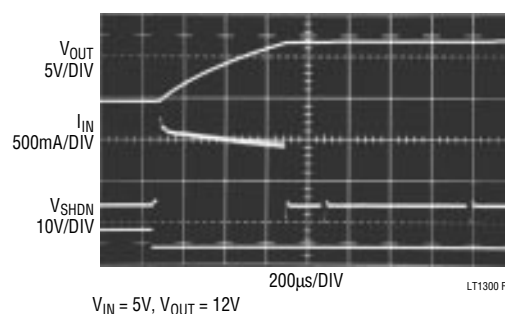
Figure 5. Start-Up Response
