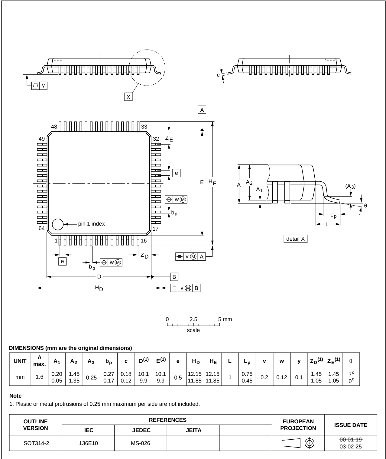
Fig 31. LQFP64 Package outline
