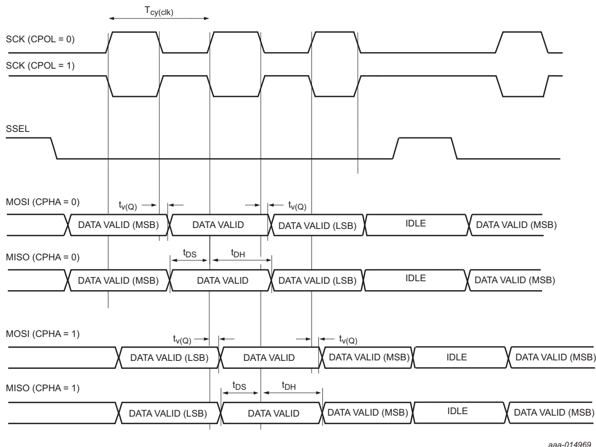
Fig 21. SPI master timing
