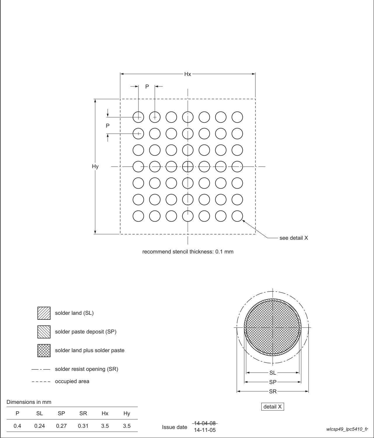
Fig 32. WLCSP49 Soldering footprint
