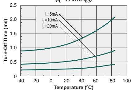
Typical Turn-Off Time vs. Temperature ( I_L=170\text{mA}_{DC} )
