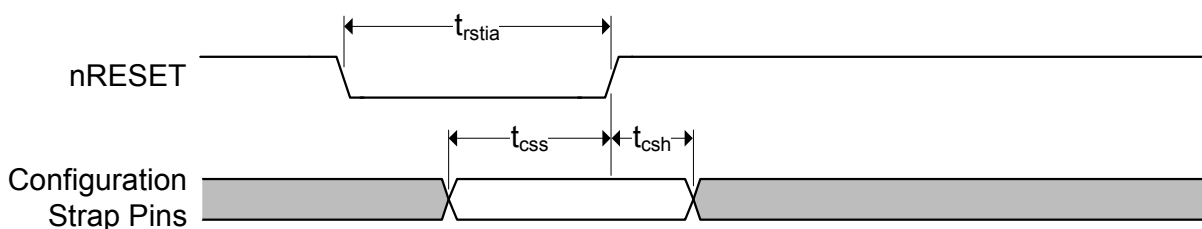
Figure 6.7 nRESET Reset Pin Timing
