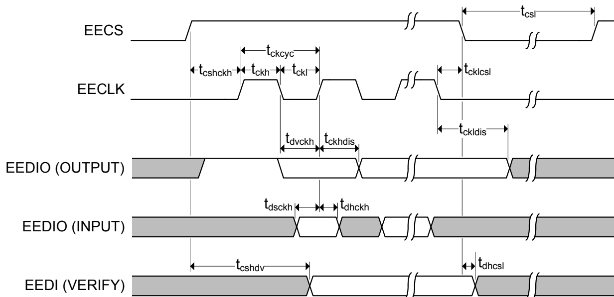
Figure 6.8 EEPROM Timing
