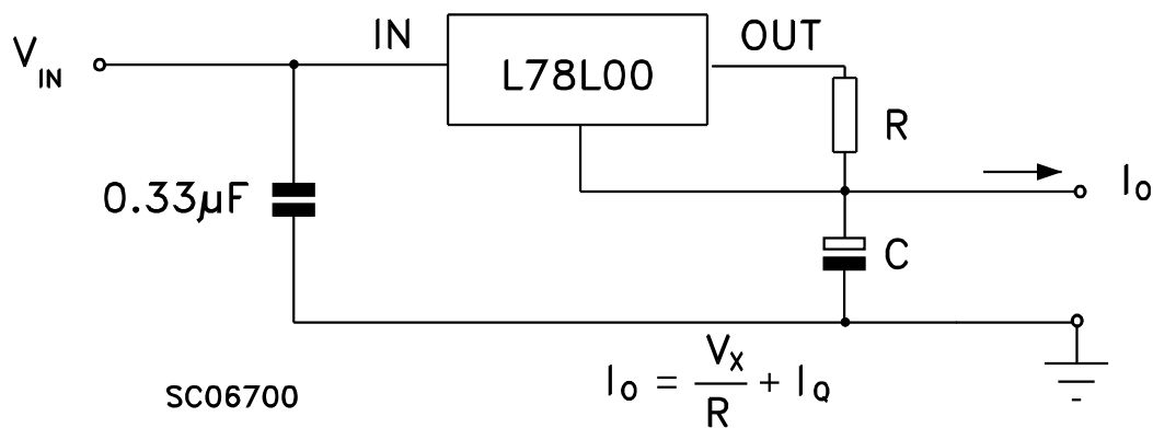
Figure 15. Current regulator
