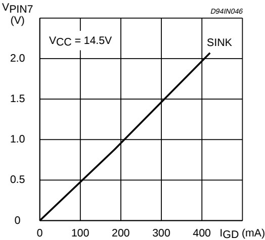
Figure 15. Output Saturation Voltage vs. Sink Current
