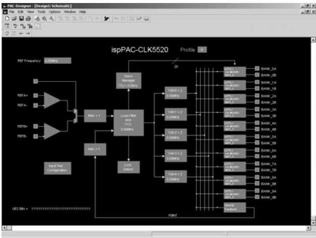
Figure 30. PAC-Designer Design Entry Screen (ispClock5520)
