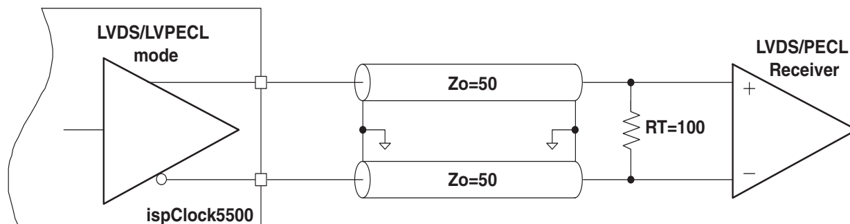
Figure 25. Configuration for LVDS and LVPECL Output Modes
