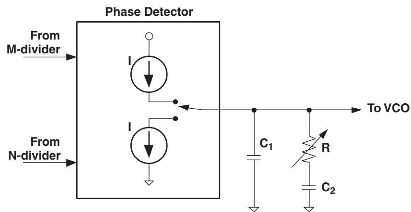
Figure 11. ispClock5500 Loop Filter (Simplified)
