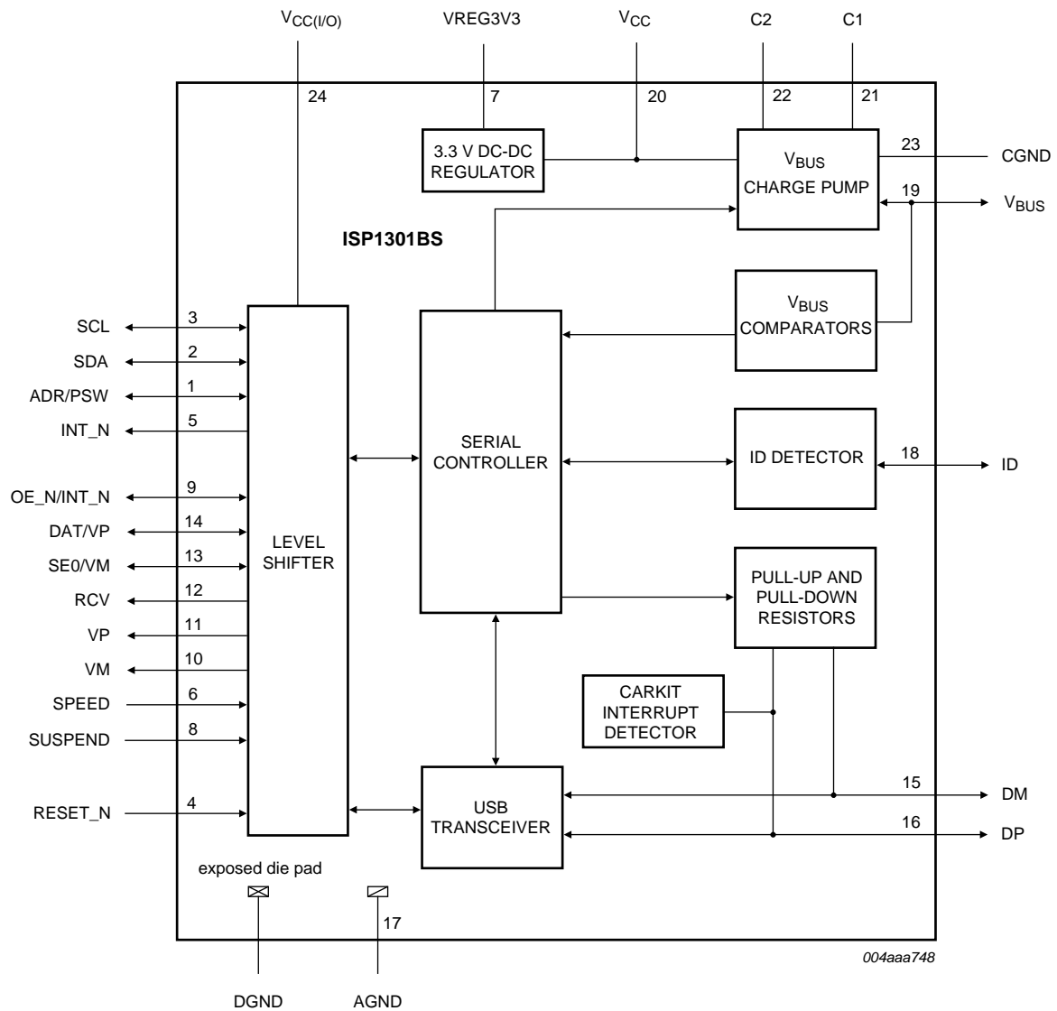
Fig 1. Block diagram
