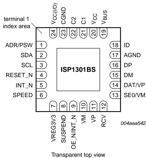
Fig 2. Pin configuration HVQFN24 (top view)
