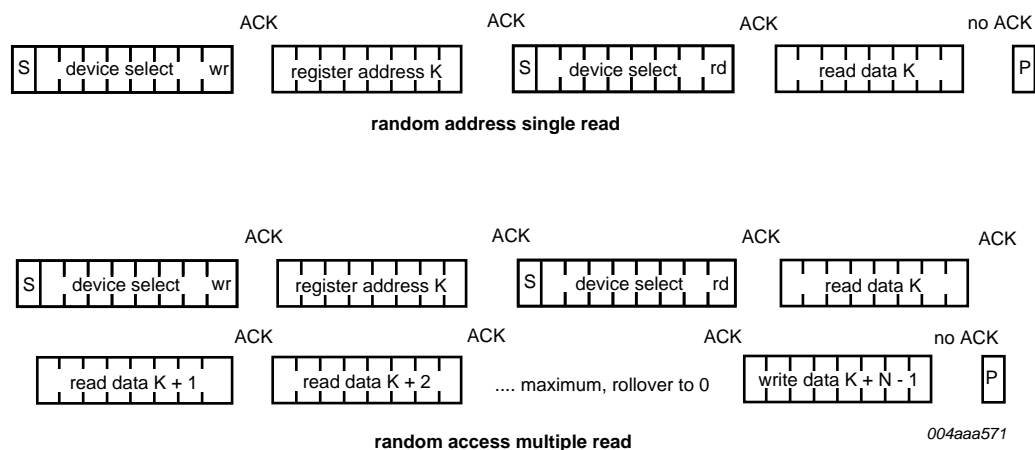
Fig 15. Random address read
