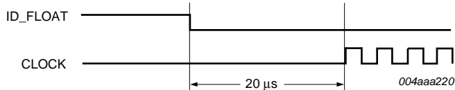
Fig 10. Clock wake-up by ID change (1)
