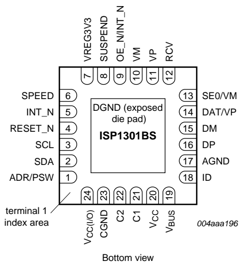
Fig 3. Pin configuration HVQFN24 (bottom view)
