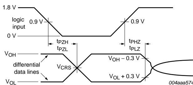
Fig 18. Timing of OE_N/INT_N to DP and DM
