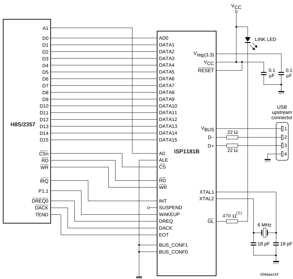
Fig 31. Typical interface circuit for bus configuration mode 0 (shared ports: 16-bit PIO, 16-bit DMA).
