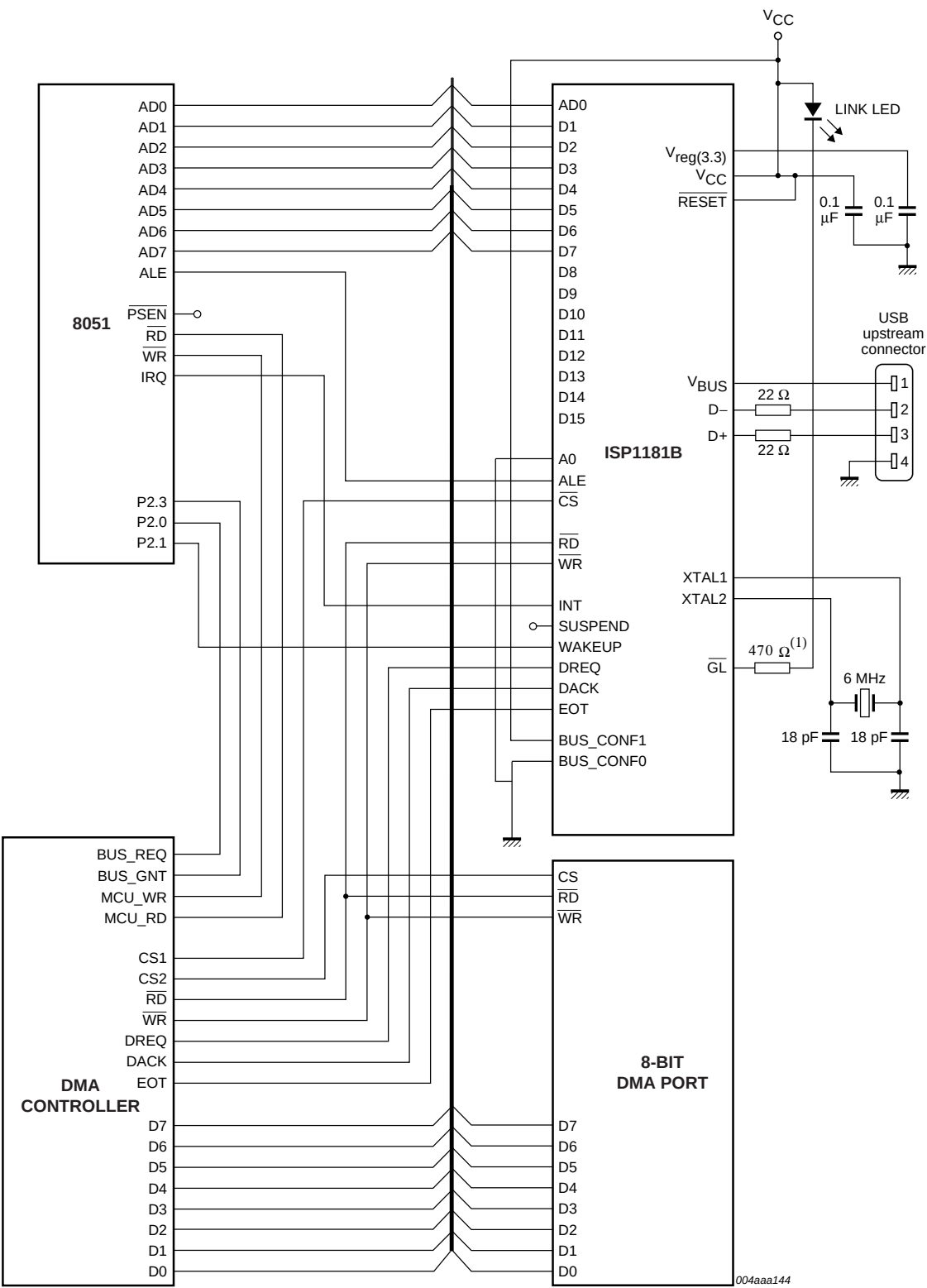
Fig 32. Typical interface circuit for bus configuration mode 2 (shared ports: 8-bit PIO, 8-bit DMA).
