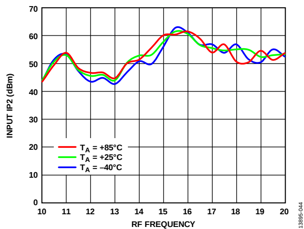
Figure 45. Input IP2 vs. RF Frequency at Various Temperatures, LO = 13\text{ dBm}
