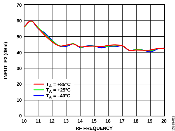
Figure 23. Input IP2 vs. RF Frequency at Various Temperatures, LO = 13\text{ dBm}
