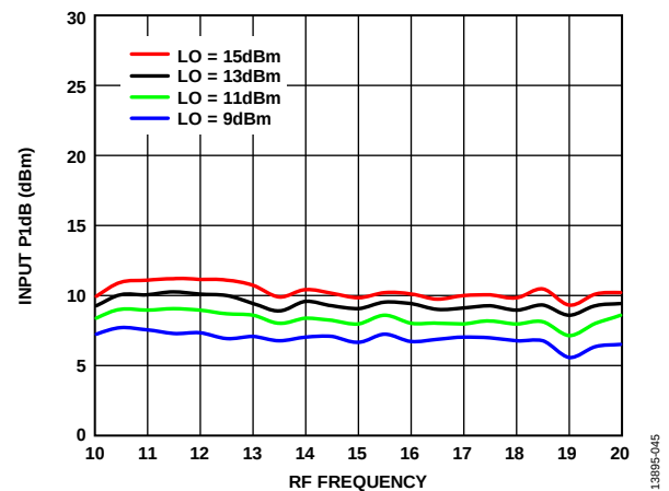
Figure 44. Input P_{1\text{dB}} vs. RF Frequency at Various LO Power Levels, T_A = 25^\circ\text{C}
