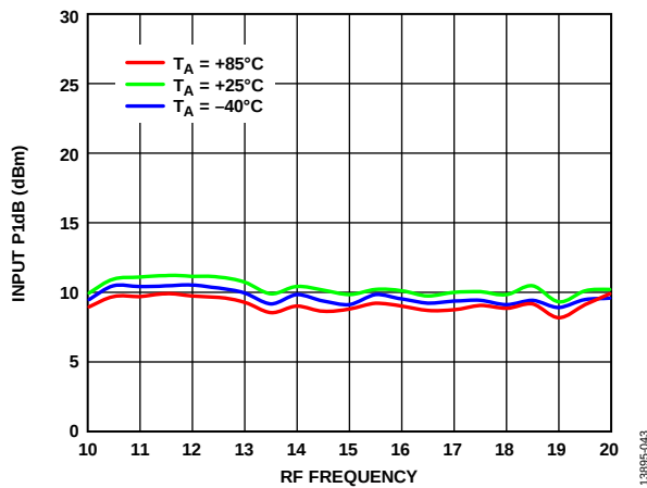
Figure 41. Input P_{1\text{dB}} vs. RF Frequency at Various Temperatures, LO = 13 dBm
