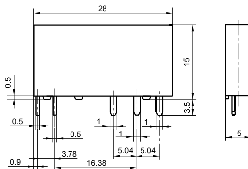
1 Form C
