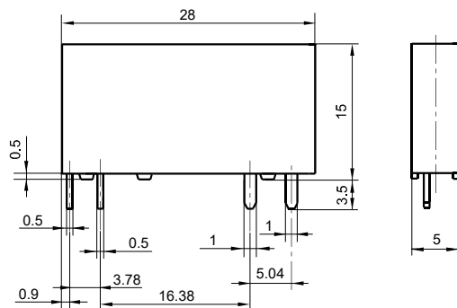
1 Form A
