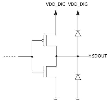
Figure 3-4: SDOUT
