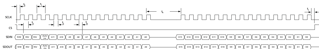
Figure 4-14: GSPI Write Mode Timing
