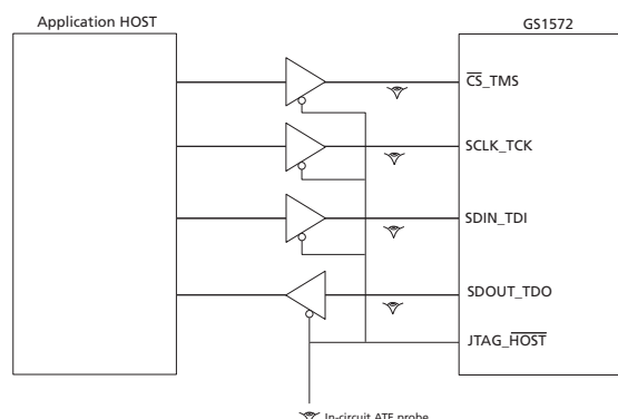
Figure 4-15: In-Circuit JTAG
