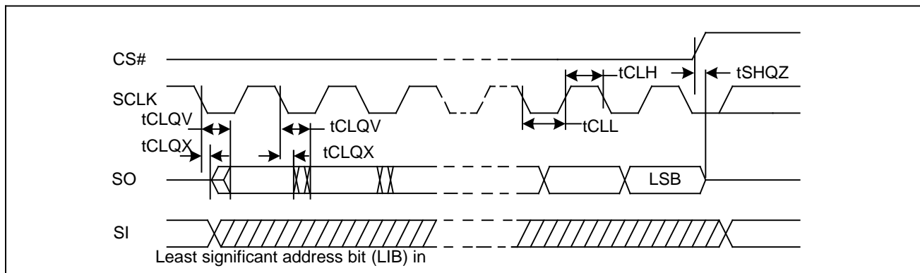
Figure 39. Output Timing
