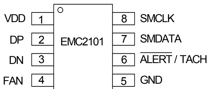
Figure 2.1 EMC2101 Pinout
