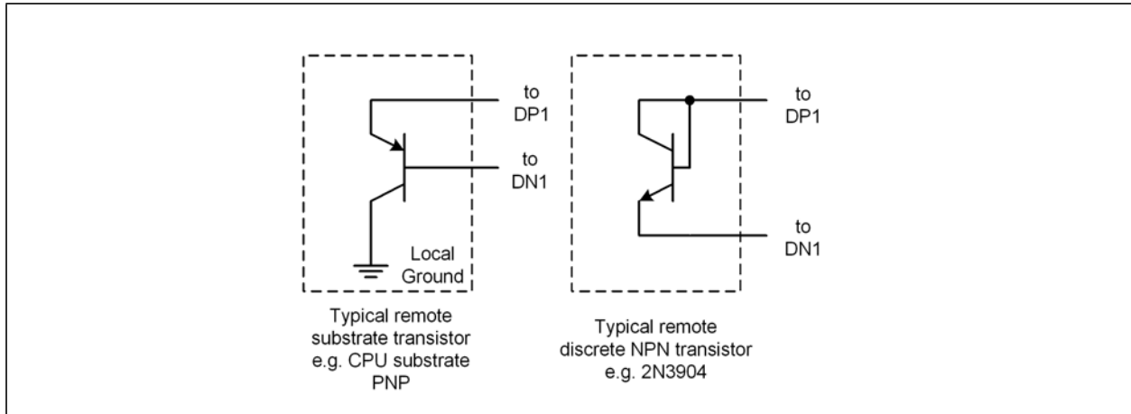
Figure 6.4 Diode Configurations
