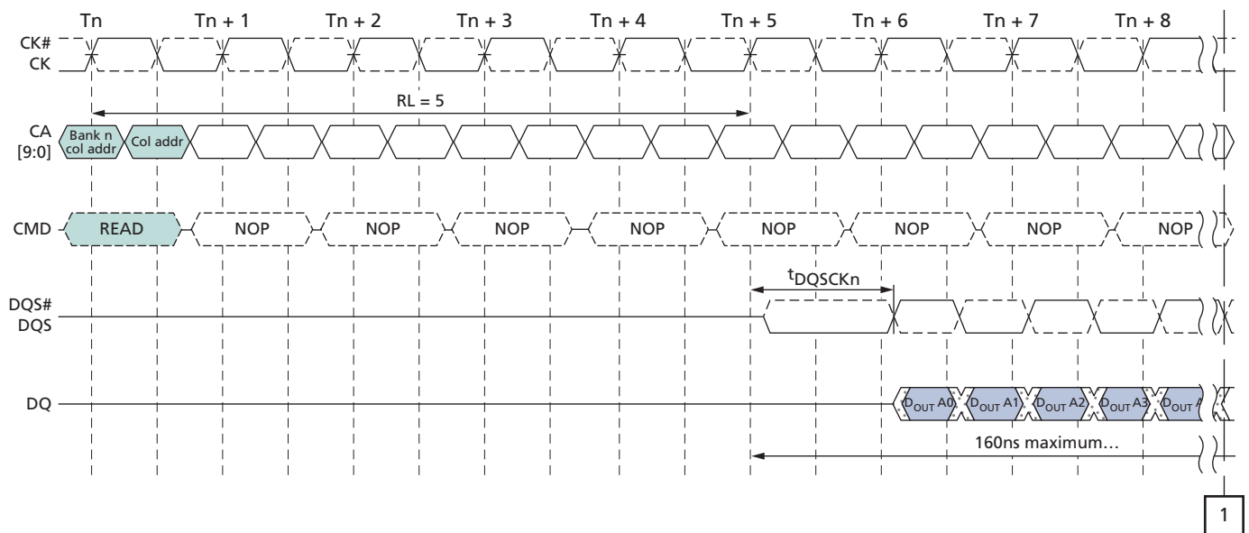
Figure 24: t_{DQSKDS} Timing
