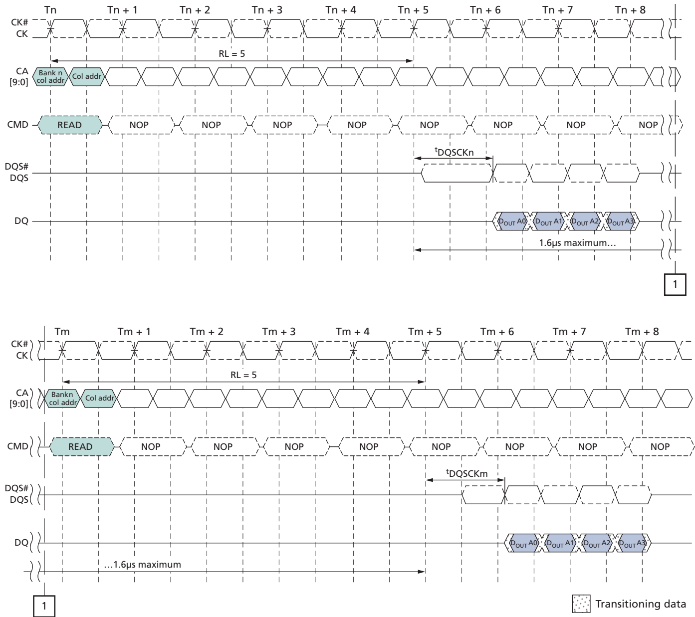
Figure 23: t_{DQSKDM} Timing
