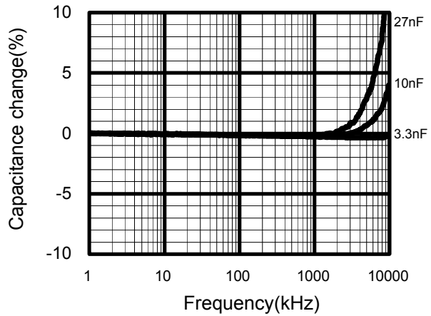
Frequency Characteristics
