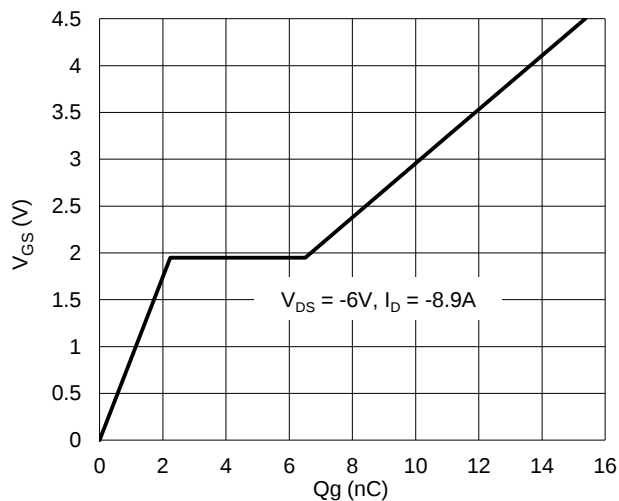
Figure 23. Gate Charge
