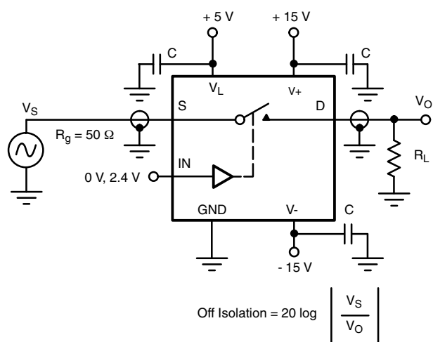
Figure 7. Off Isolation
