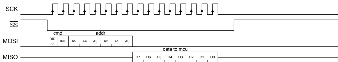
Figure 5. SPI Incrementing Burst Read Sequence
