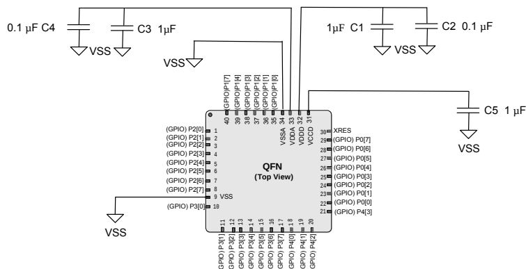
Figure 12. 40-pin QFN Example
