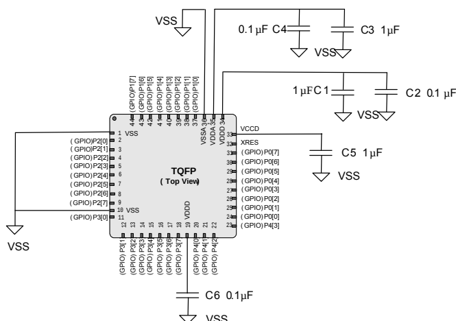
Figure 11. 44-TQFP Package Example
