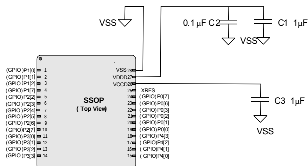
Figure 13. 28-SSOP Example
