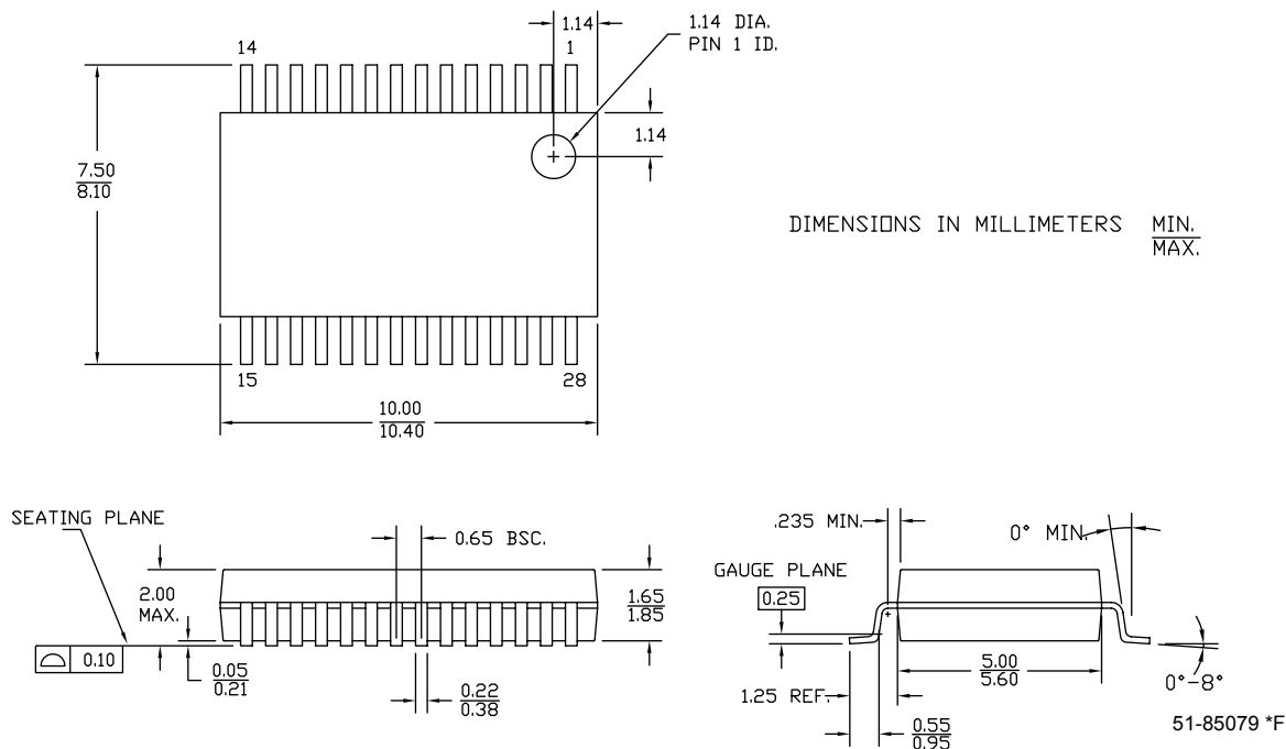
Figure 14. 28-pin (210-mil) SSOP Package Outline
