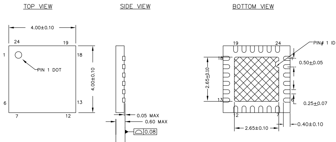
Figure 20. 24-Pin (4 × 4) QFN (Sawn)
