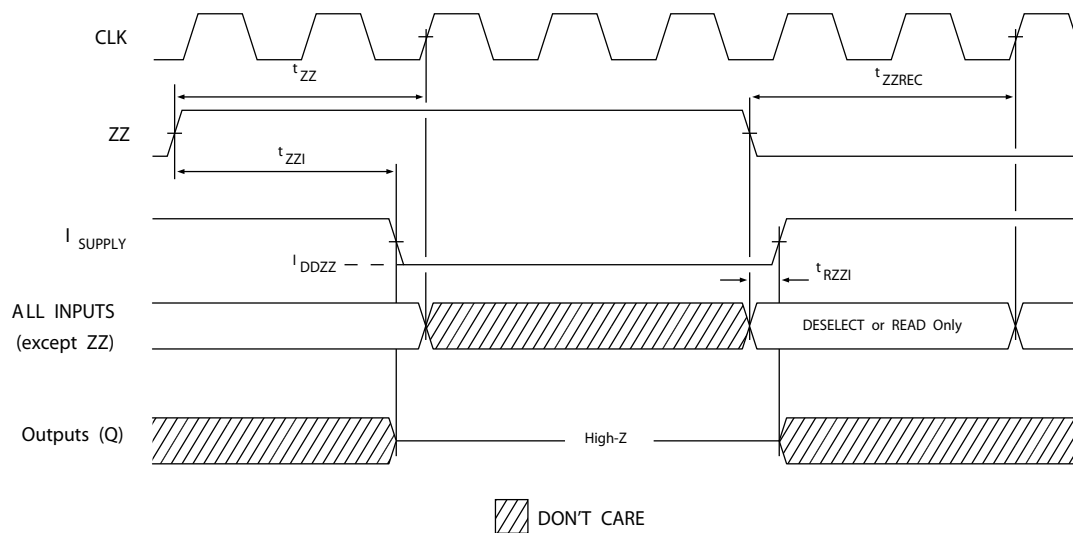
Figure 7. ZZ Mode Timing [33, 34]
