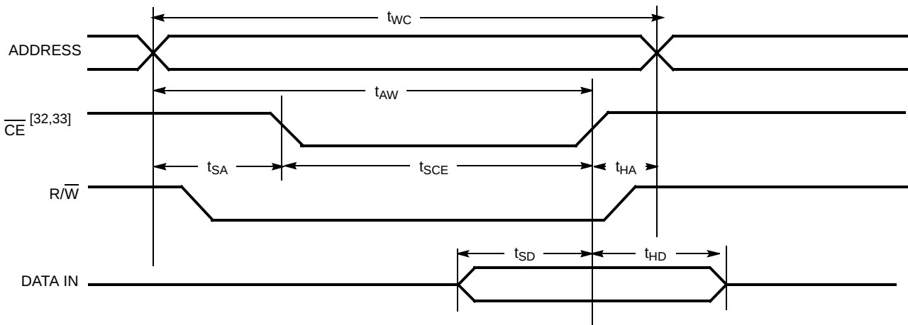
Figure 8. Write Cycle No. 2: \overline{CE} Controlled Timing [28, 29, 30, 36]
