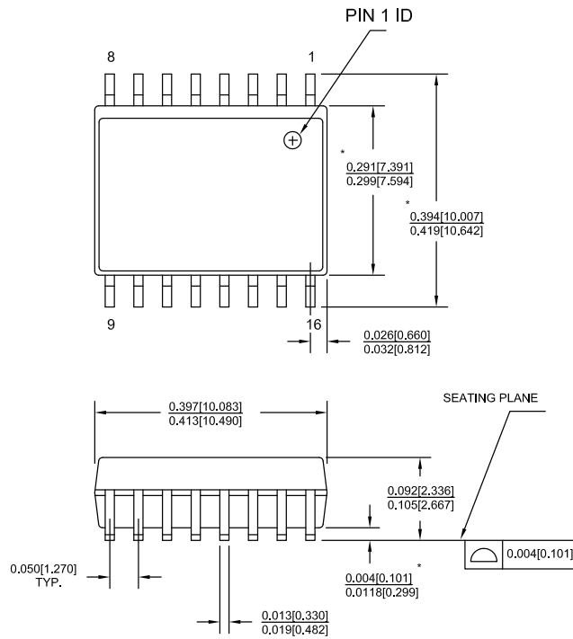
Figure 33. 16-pin SOIC (0.413 × 0.299 × 0.0932 inches) Package Outline, 51-85022
