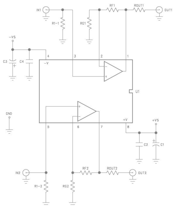
Figure 9. CEB006 &amp; CEB010 Schematic
