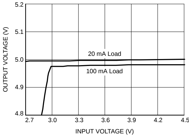
Figure 5. Line Regulation
