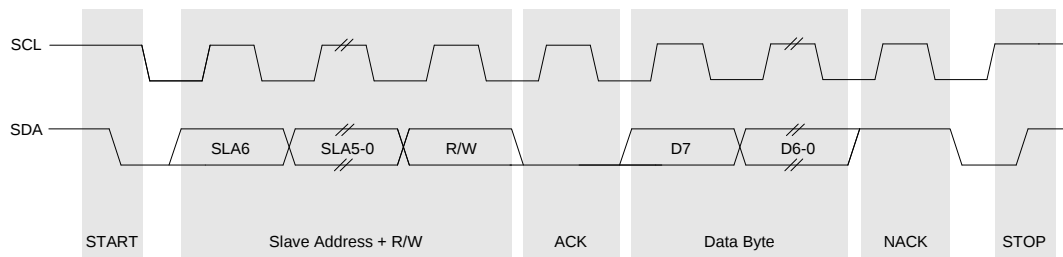
Figure 17.3. SMBus Transaction
