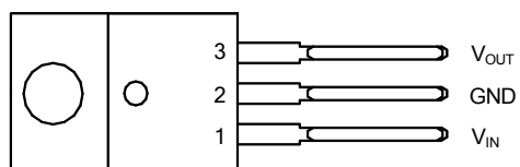
T Package (TO-220-3)
