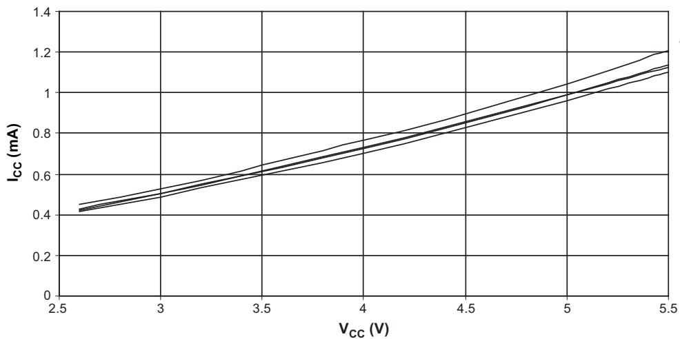
Figure 23-6. Active Supply Current versus V_{CC} (Internal RC Oscillator, 1MHz)
