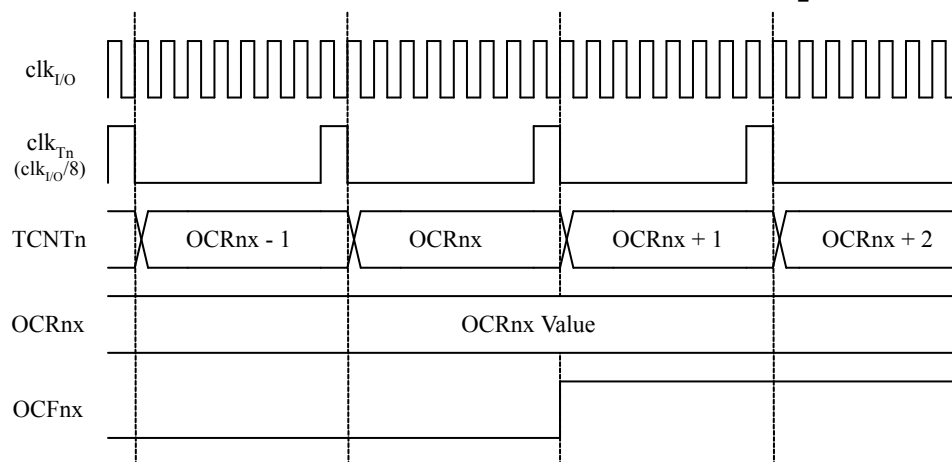
Figure 13-13 Timer/Counter Timing Diagram, Setting of OCF0x, with Prescaler ( f_{\text{clk\_I/O}}/8 )
