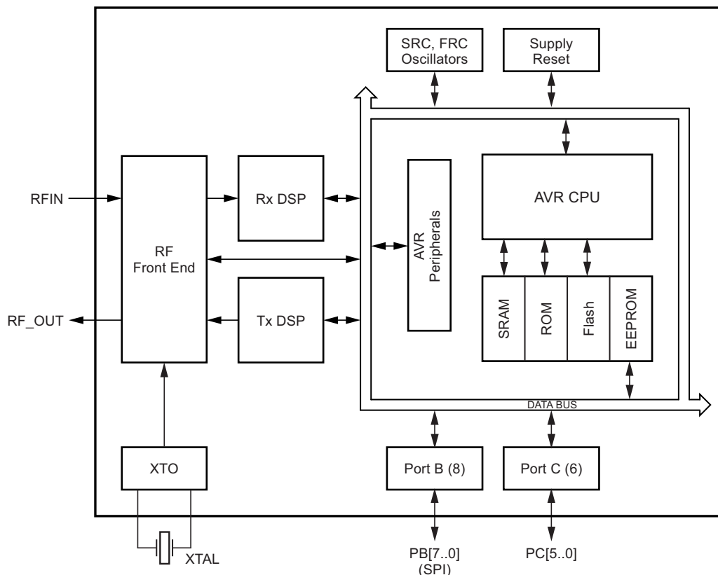
Figure 1-1. Circuit Overview
