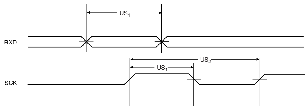
Figure 6. USART Signals
