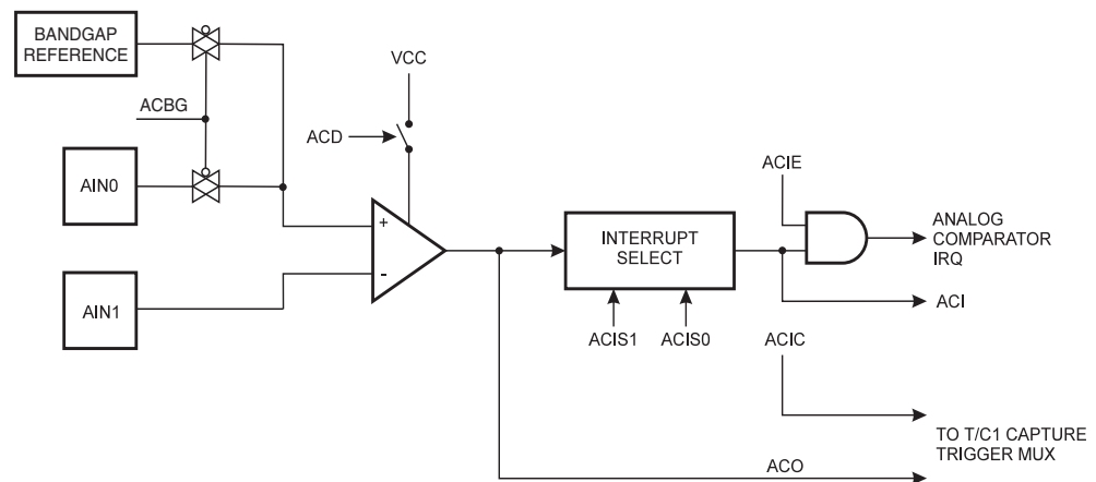
Figure 22-1. Analog Comparator Block Diagram (1)
