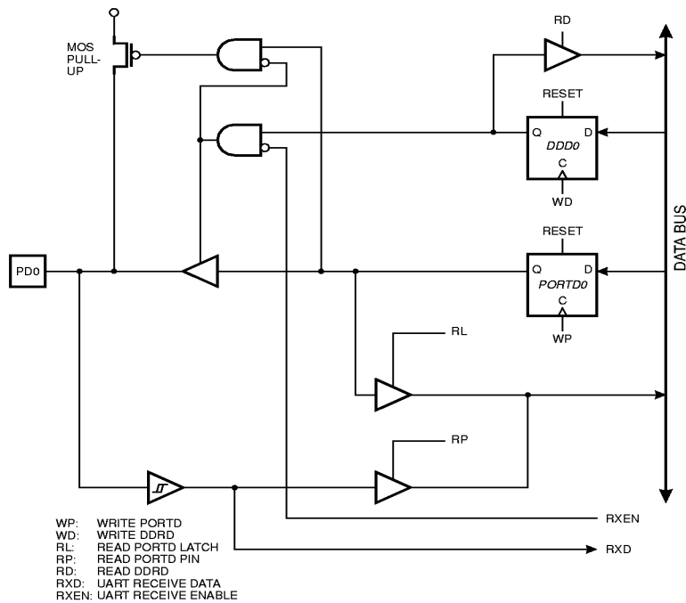
Figure 57. PORTD Schematic Diagram (Pin PD0)
