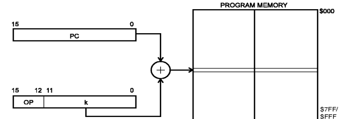
Figure 18. Relative Program Memory Addressing
