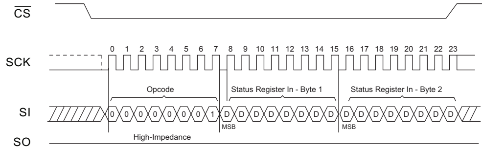
Figure 10-3. Write Status Register
