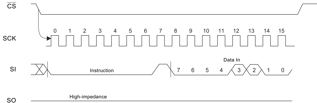
Figure 7-5. WRSR Timing
