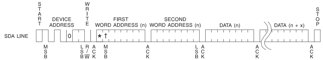
Figure 9. Page Write
