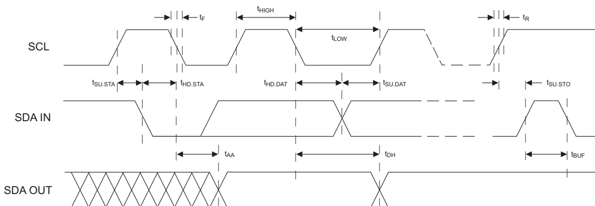
Figure 8-1. Bus Timing
