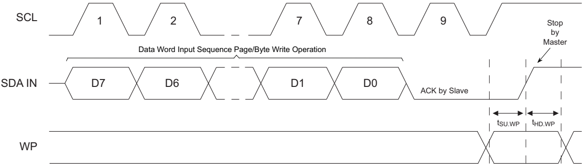
Figure 5-5. Write Protect Setup and Hold Timing
