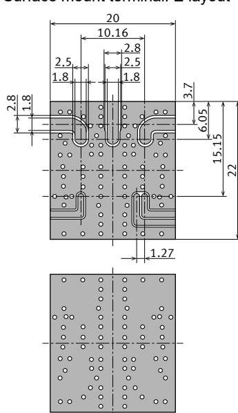
Surface mount terminal: E layout
