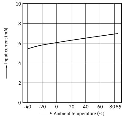
8. Input current vs. ambient temperature characteristics
