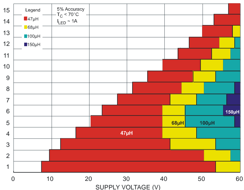
Figure. 16 Recommended Inductor with 1A LED Current
