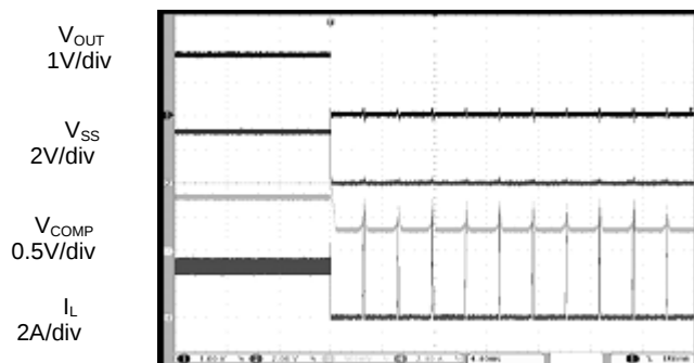
Short Circuit Protection ( V_{IN}=5V , V_{OUT}=1.8V , I_{OUT}=3A )
