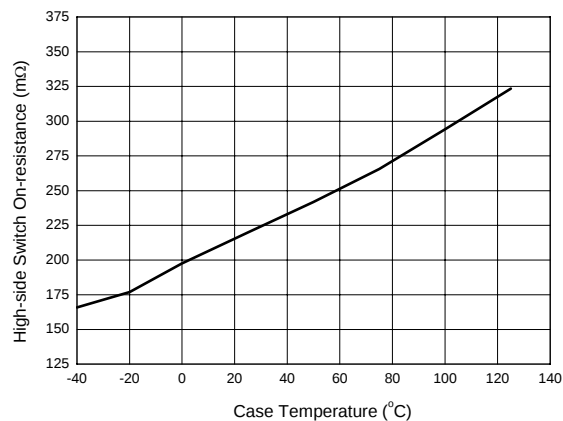
Figure 5. R_{\text{DS(on)H}} vs. Case Temperature
