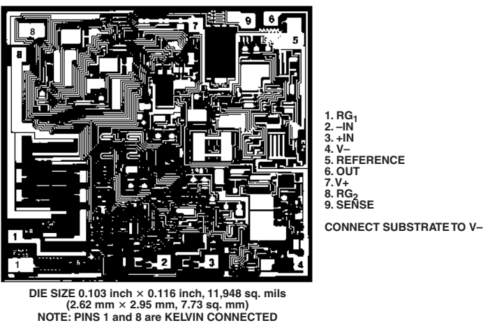
Die Characteristics
