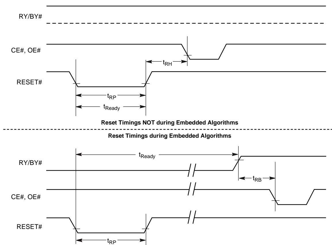
Figure 14. Reset Timings
