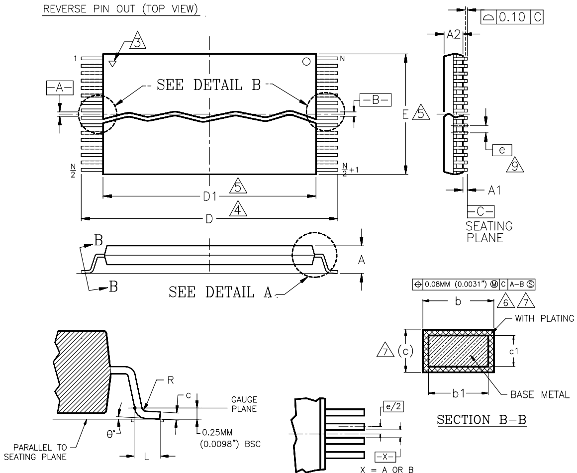
DETAIL A
