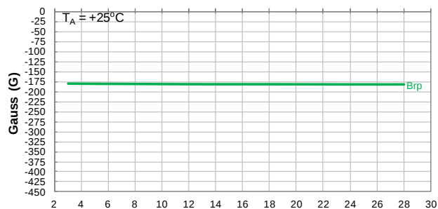
Switch Release Point B_{rp} vs Supply Voltage
