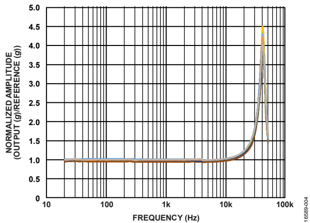
Figure 4. Frequency Response, High Frequency (>5 kHz) Vibration Response; a Laser Vibrometer Controller Referencing the ADXL1005 Package Used for Accuracy
