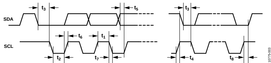
Figure 3. I²C Timing
