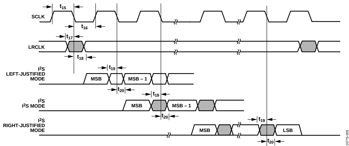
Figure 5. I²S Timing
